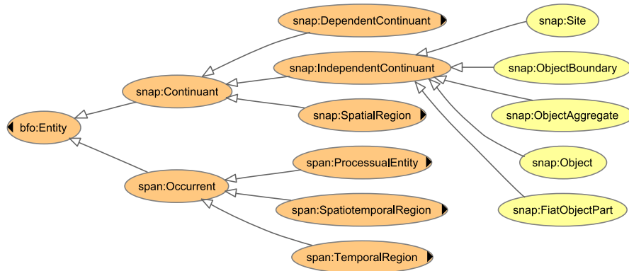
Figure 1. Excerpt from the BFO class tree
